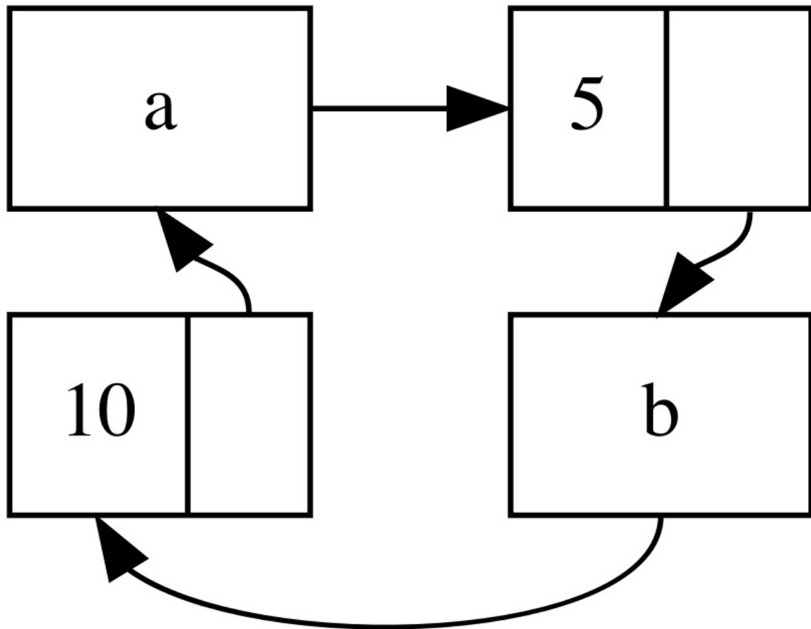
Figure 15-4: A reference cycle of lists a and b pointing to each other
